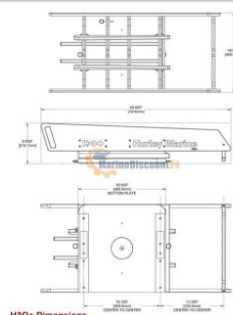
H30+ Dimensions
